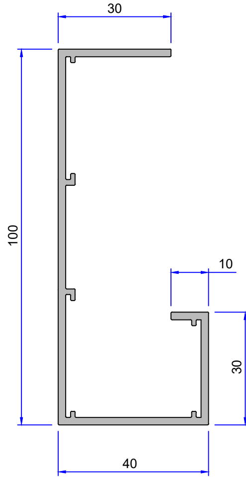
Profile Detail
