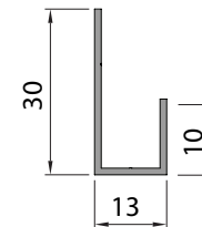
SKR HANGING STRIP
