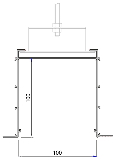
BBOX100/TP FULL CEILING TILE TO PLASTERBOARD
