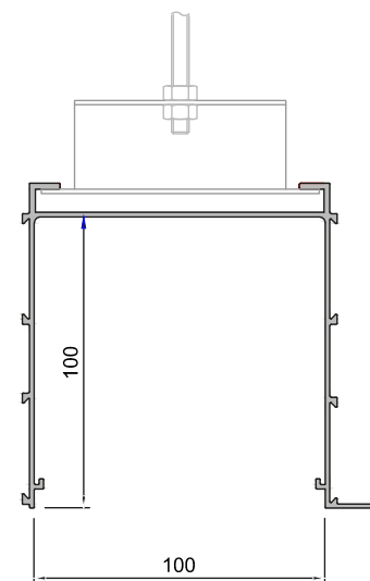
BBOX100/WT WALL TO FULL CEILING TILE
