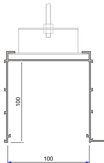
BBOX100/WP WALL TO PLASTERBOARD
