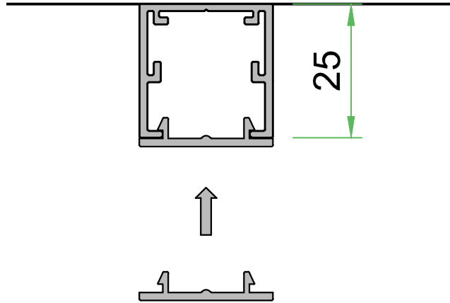
INSTALLATION DETAIL Scale: 1:2
