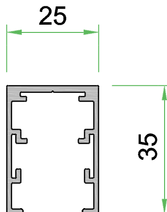
SGHT35 PROFILE Scale: 1:1
