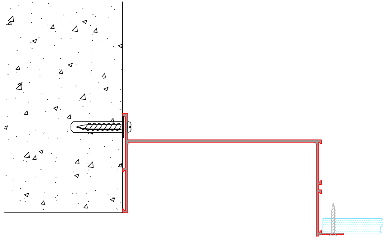
BBOX160X80 - INSTALLATION DETAIL Scale: 1:2
