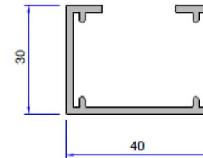
Profile Detail
