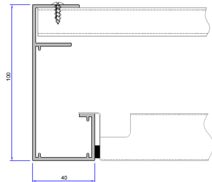
Installation Detail
