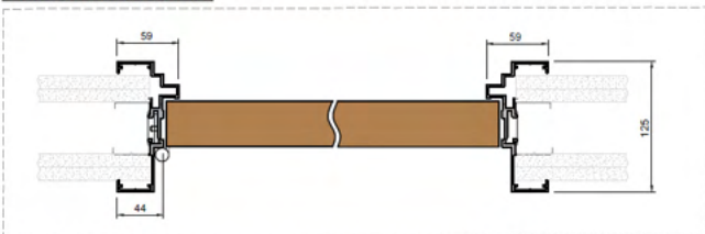
DOUBLE GLAZED DOOR FRAME DETAILS
