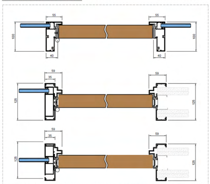
SINGLE GLAZED DOOR FRAME DETAILS
