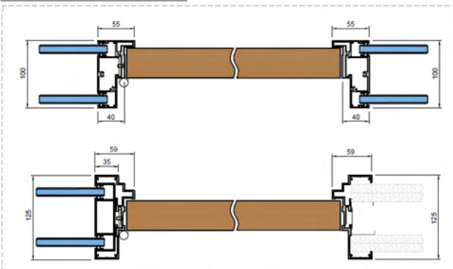
DOUBLE GLAZED DOOR FRAME DETAILS
